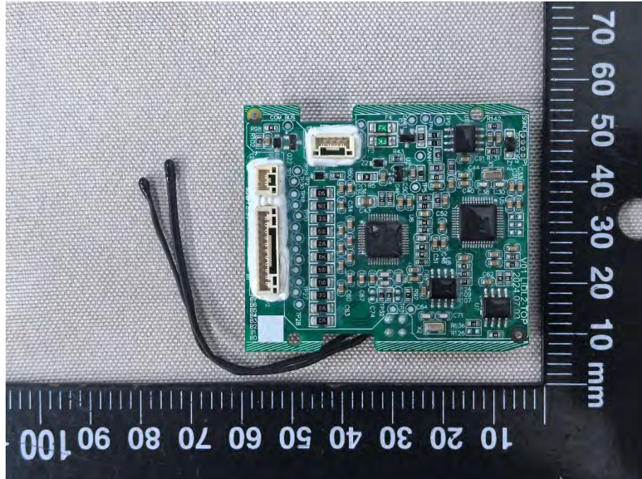
Picture 7 Rear View of PCM A
