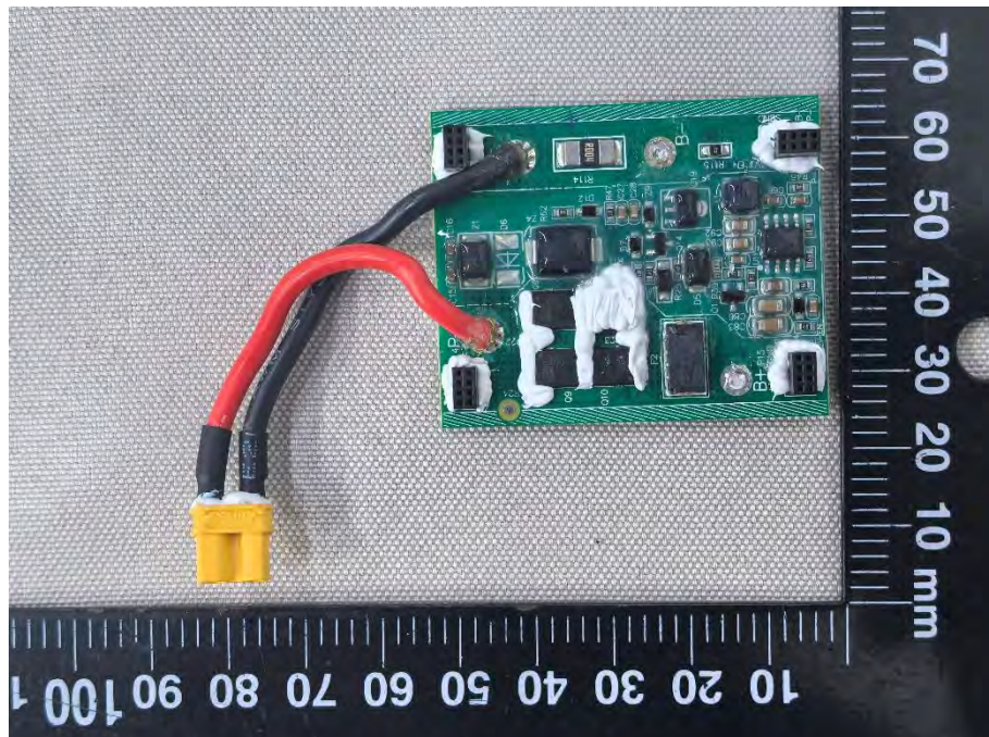
Picture 8 Front View of PCM B
