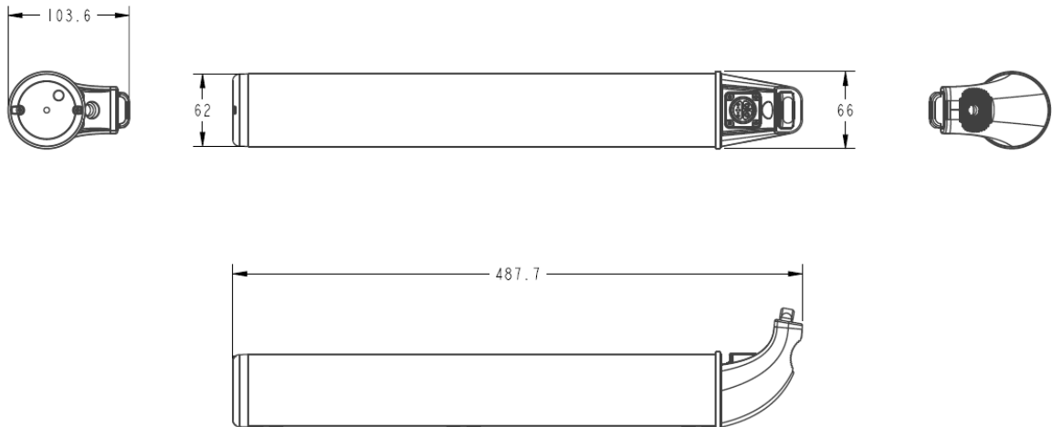
Battery (unit: mm)
