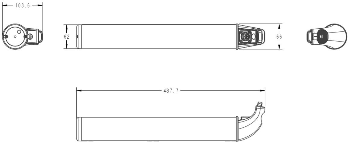
Battery (Unit: mm)
