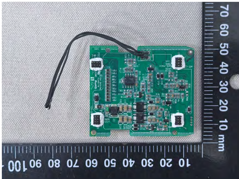
Picture 6 Front View of PCM A
